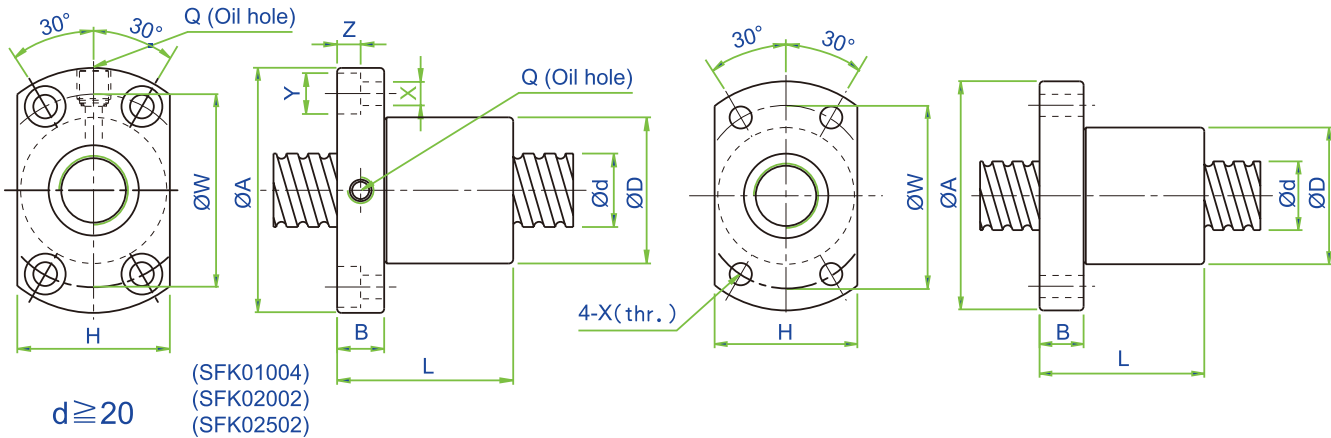
SFK Series Specifications
