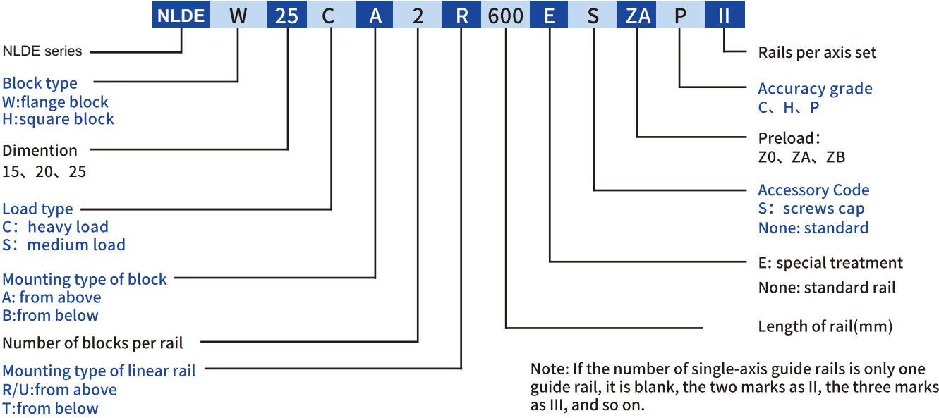
Interchangeable linear guide product model
