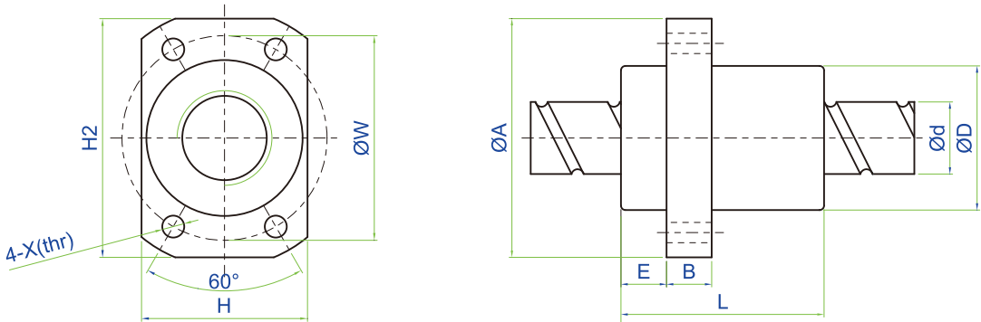
XSY Series Specifications
