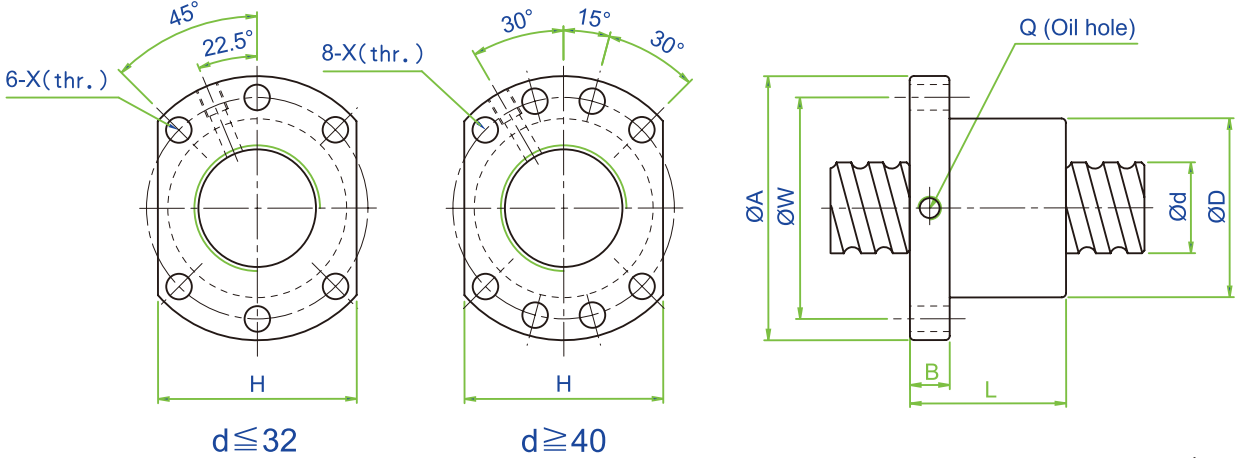
SFNU/SFU (DIN 69051 FORM B) Series Specifications
