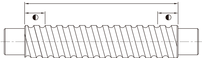
Fig 3.6.5 Harden Area
