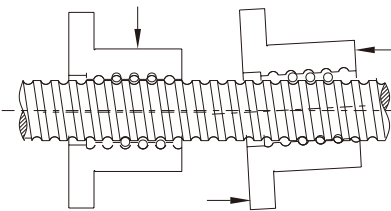
Fig 3.6.3 Offset Load
