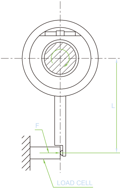
Fig 3.3.4 Preload dynamic torque measuring method
