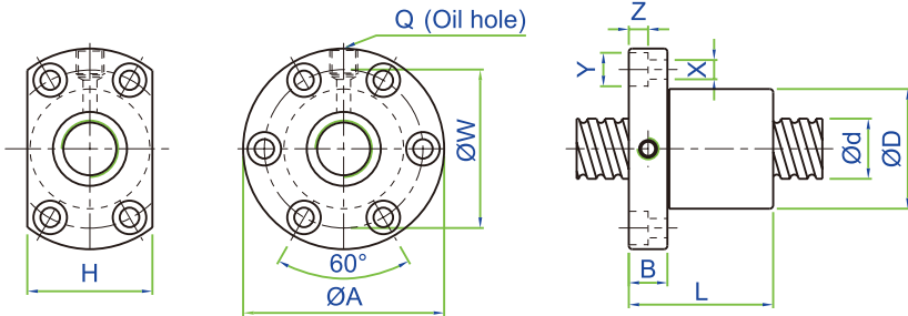
SFM Series Specifications (Design for Milling)
