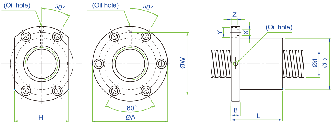
SFV Series Specifications
