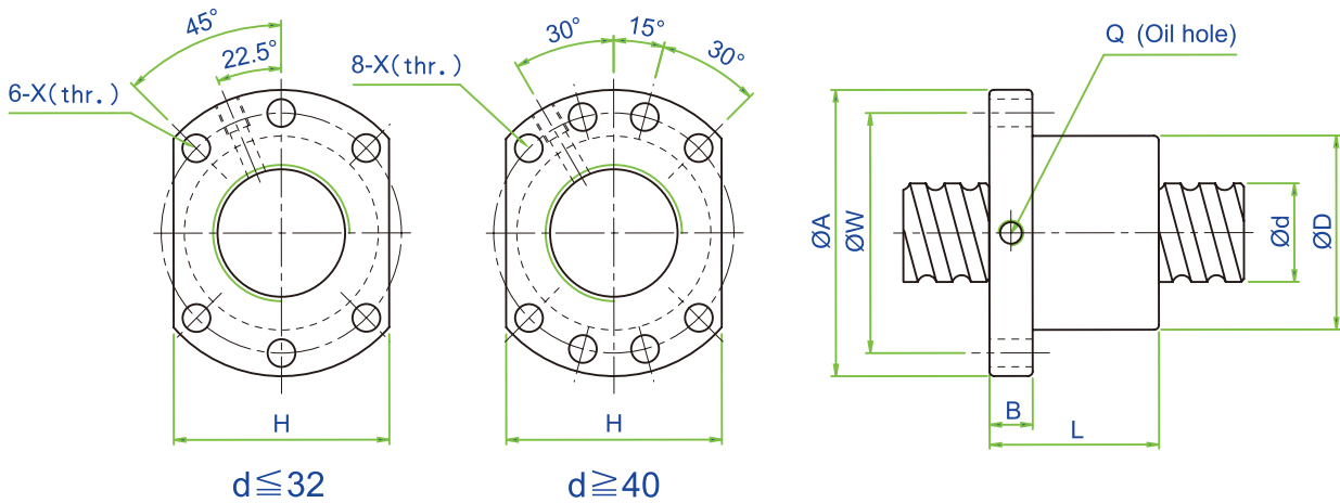
SFNU/SFU (DIN 69051 FORM B) Series Specifications
