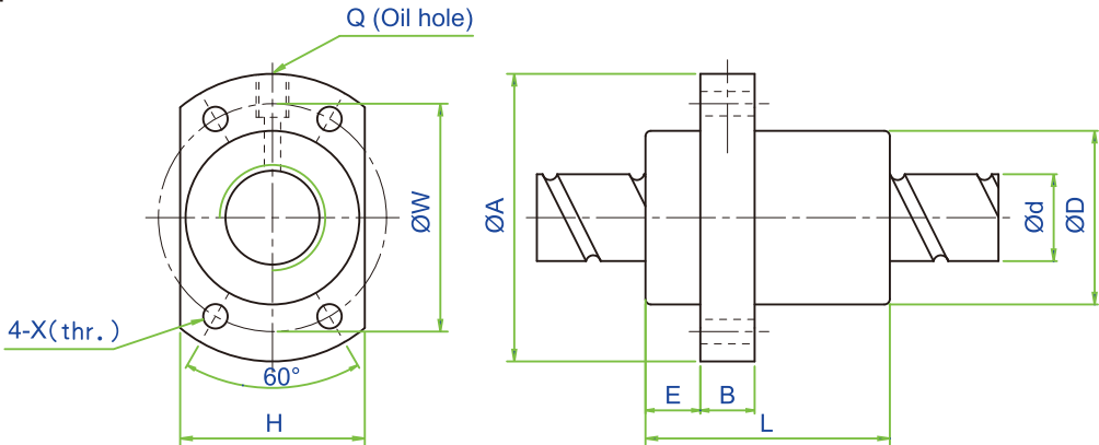
SFY Series Specifications
