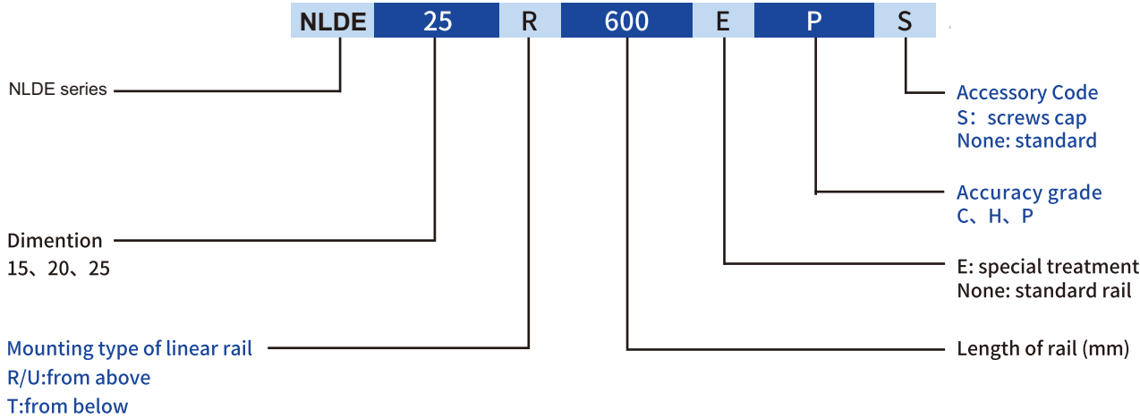
Interchangeable type rail product model
