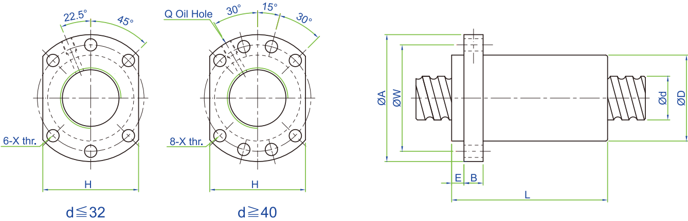
SFA Series Specifications
