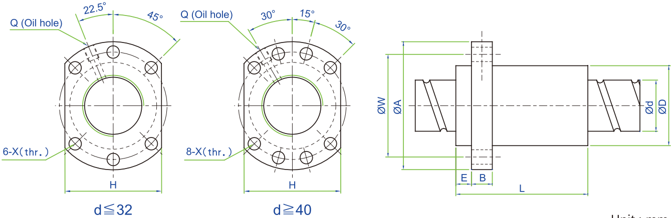
SFNH/SFH (DIN 69051 FORM B) Series Specifications
