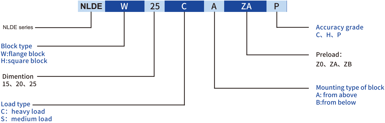
Interchangeable type block product model
