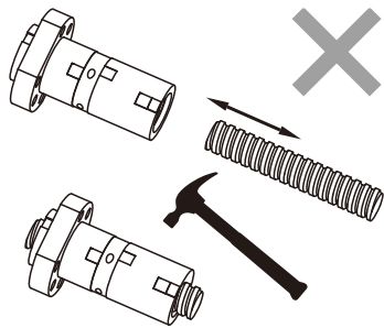
Fig 3.6.1 Error installation
