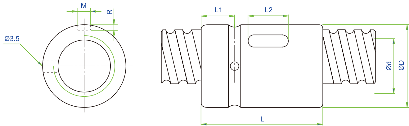
SCNI/SCI Series Specifications
