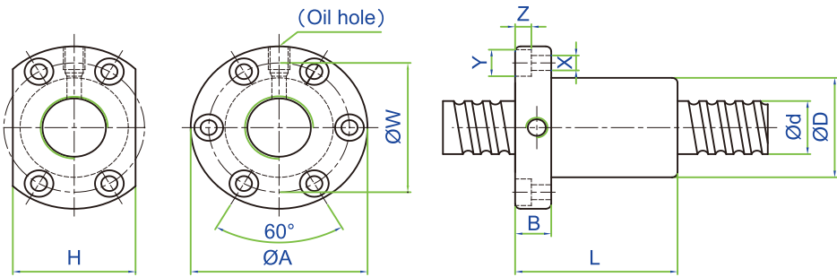
SFNI/SFI Series Specifications
